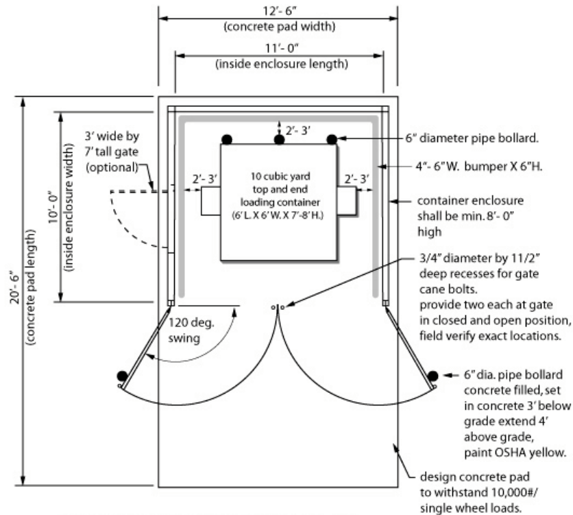
CONTAINER ENCLOSURE PLAN
